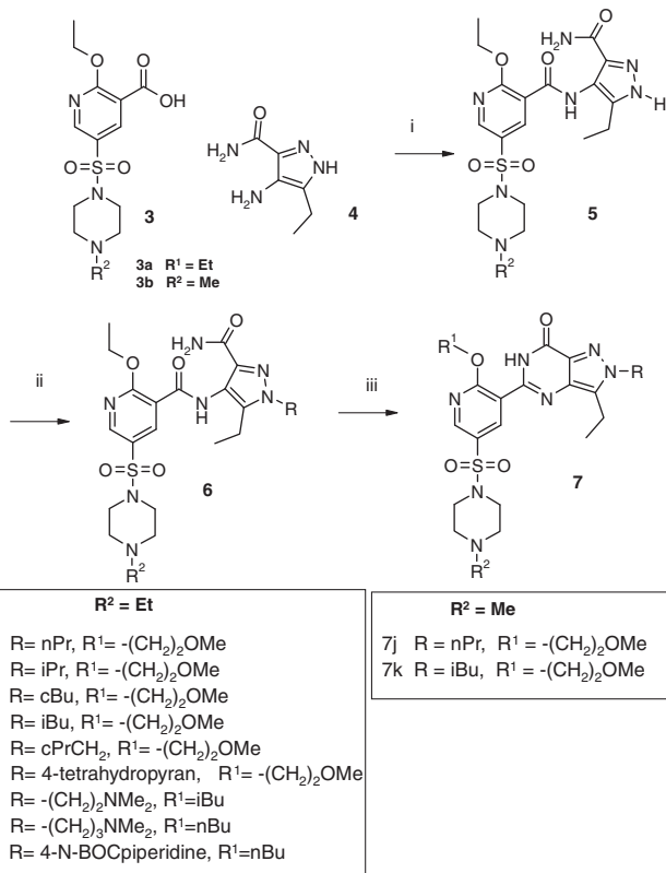
Scheme 1. Reagents and conditions: (i) 1-(3-dimethylaminopropyl)-3-ethyl-carbodiimide hydrochloride, hydroxybenzotriazole, di-isopropylethylamine, THF, 20 °C, 20 h; (ii) caesium carbonate, alkyl mesylate or alkyl chloride, DMF, 20 °C, 20 h; (iii) KHMDS, R 1 OH, 120 °C, 20 h.
