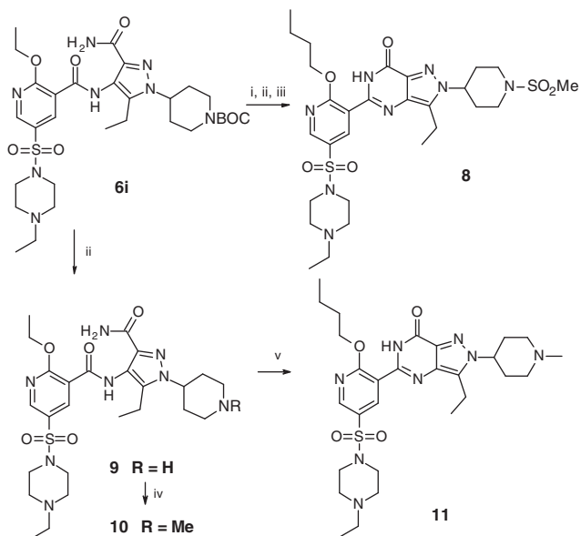
Scheme 2. Reagents and conditions: (i) KHMDS, n BuOH, 120–130 °C, pressure vessel (ii) TFA, CH 2 Cl 2 ; (iii) methanesulphonyl chloride, NEt 3 , CH 2 Cl 2 ; (iv) HOAc, NaCNBH 3 , CH 2 O (v) KHMDS, n BuOH, reflux.
