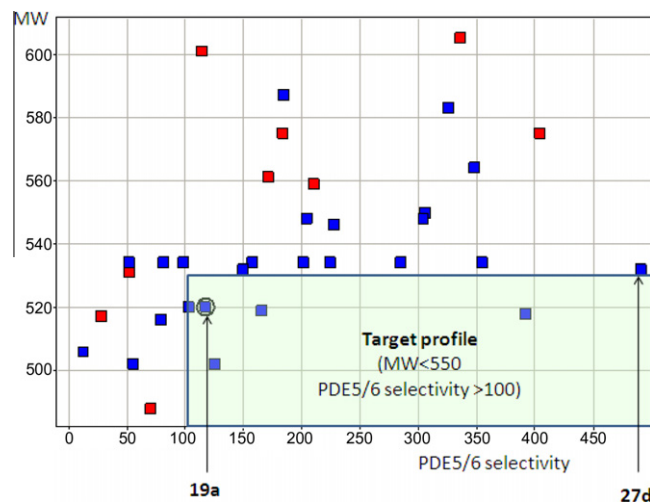
Figure 3. Effect of MW on PDE5/6 selectivity. Red spots represent the dibasic examples in Table 3. Blue spots are the monobasic examples in Tables 1–4.
