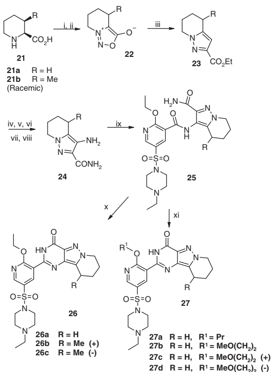
Scheme 4. Reagents and conditions: (i) NaNO 2 , HCl, H 2 O; (ii) TFAA, Et 2 O; (iii) ethyl propynoate, xylene, reflux, 2 h; (iv) NaOH, H 2 O, dioxan; (v) HNO 3 /H 2 SO 4 , 40–55 °C; (vi) (COCl) 2 , CH 2 Cl 2 , DMF; (vii) NH 3 , THF; (viii) 10% Pd/C, EtOH, 60 psi H 2 , 20 °C, 14 h; (ix) acid chloride of 3 , NEt 3 , CH 2 Cl 2 ; (x) KHMDS, EtOH, 130 °C, 14 h, pressure vessel; (xi) methoxyethanol, KHMDS, reflux, 14 h.
