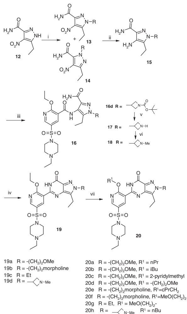
Scheme 3. Reagents and conditions: (i) caesium carbonate, RCl, DMF; (ii) 50 psi H 2 , 10% Pd/C (iii) 1-(3-dimethylaminopropyl)-3-ethyl-carbodiimide hydrochloride, HOBT, di-isopropylethylamine, THF, 20 °C, 20 h; (iv) KHMDS, ethanol, 120 °C, pressure vessel; (v) TFA, CH 2 Cl 2 ; (vi) CH 2 O, HOAc, NaCNBH 3 ; (vii) R 1 OH, KHMDS, 120 °C.
